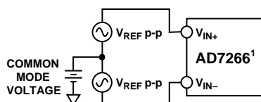
1 ADDITIONAL PINS OMITTED FOR CLARITY. 04683-020
