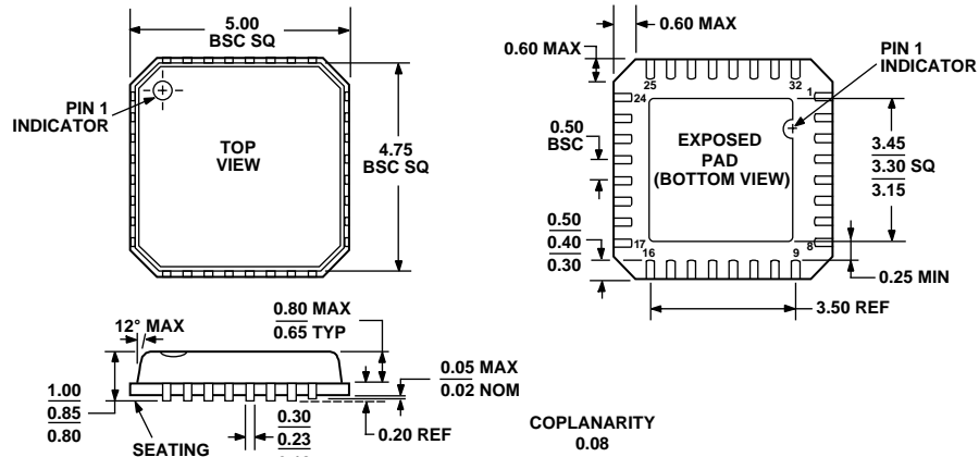
Figure 47. 32-Lead Frame Chip Scale Package [LFCSFP] (CP-32-3) Dimensions shown in millimeters
